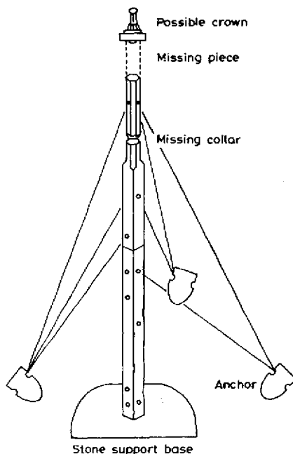
Fig. 10: Proposed reconstruction of the Dhar iron pillar according to Roessler (1995).
